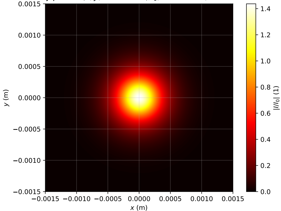
Intensity profile I(x, y, z = 0.876m)/I_0 , Pin=1.0Pcr, artificial time
